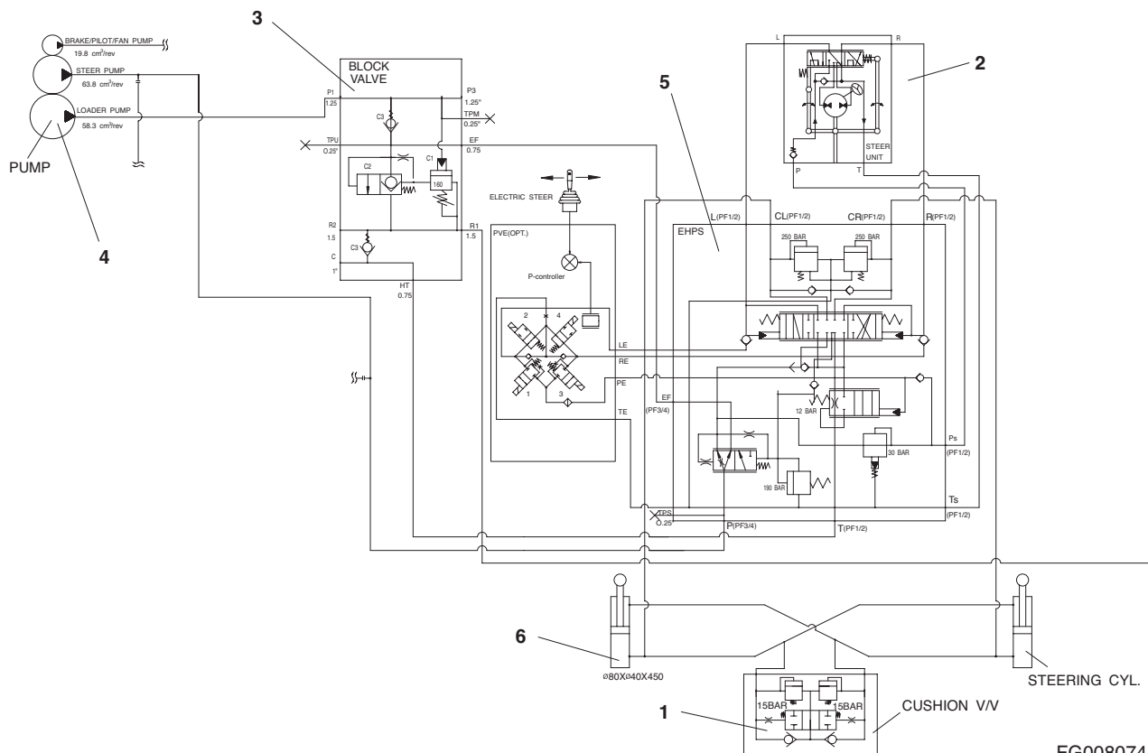
Figure 2 HYDRAULIC CIRCUIT
